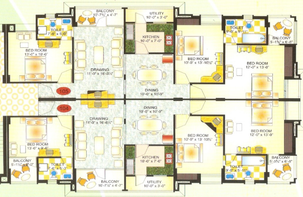
TYPICAL FLOOR PLAN (BLOCK-C)
